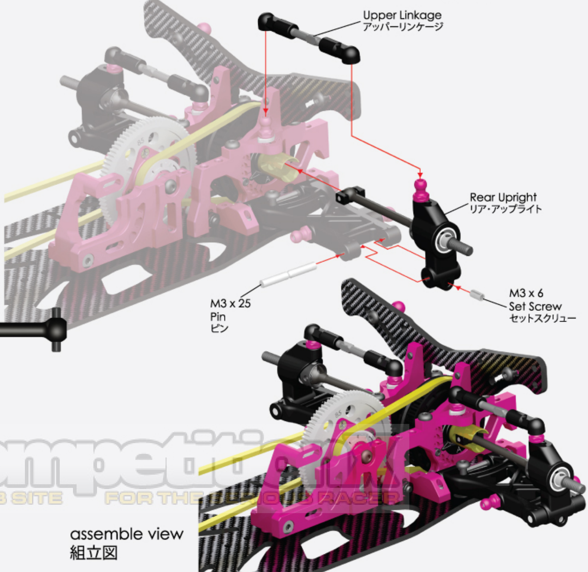
assemble view 組立図
