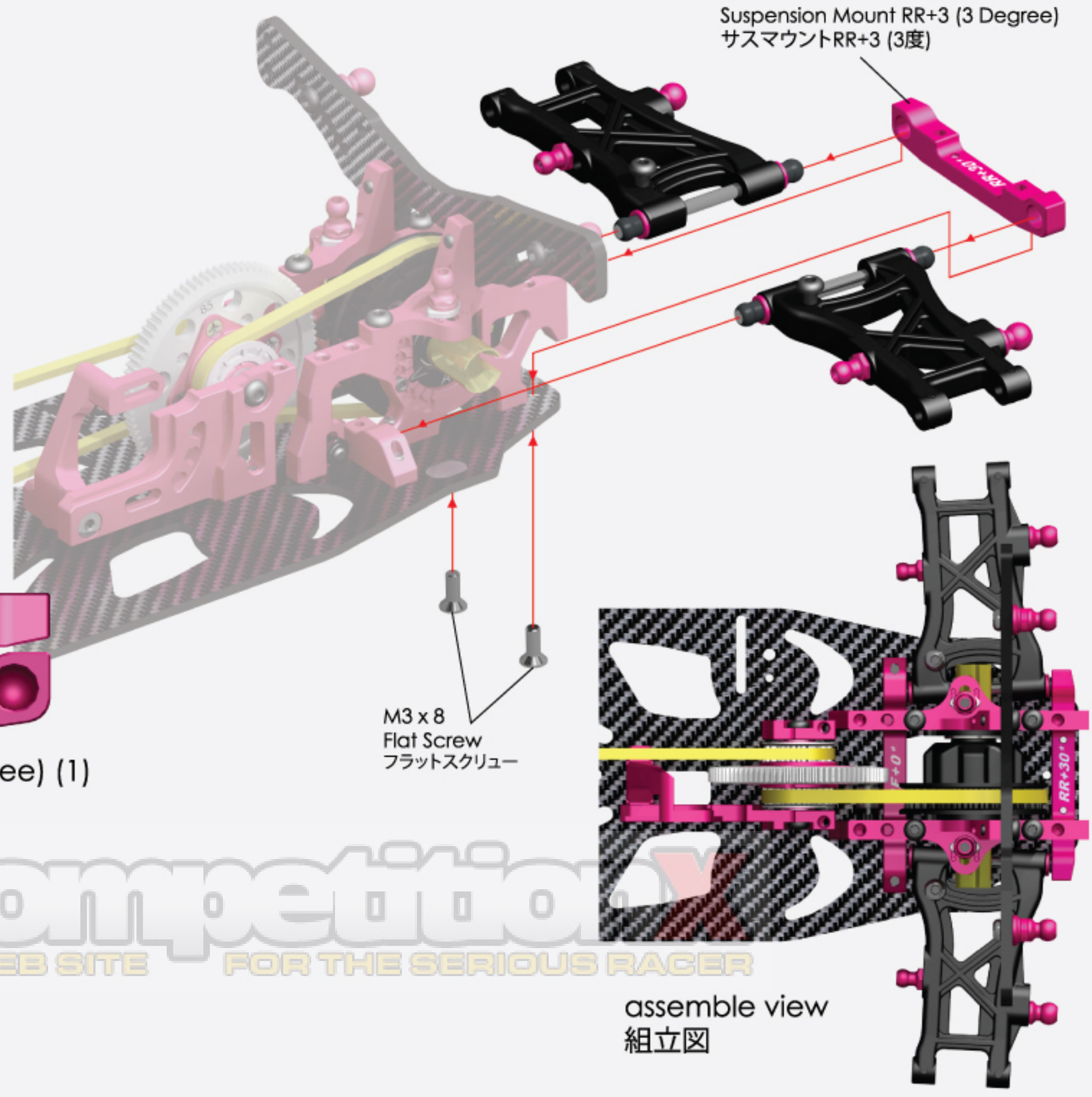
assemble view 組立図
