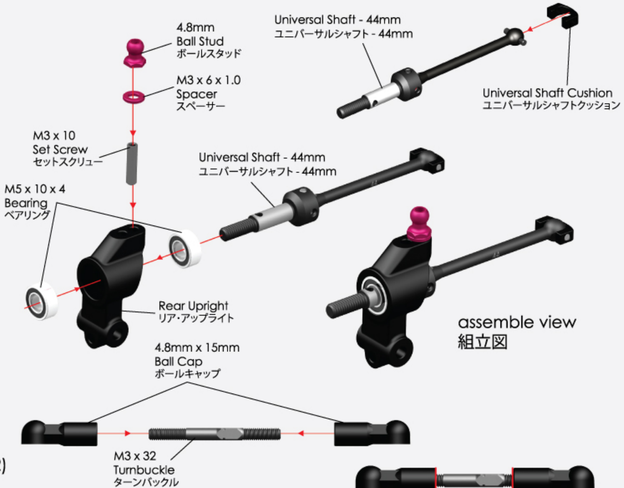
assemble view 組立図
